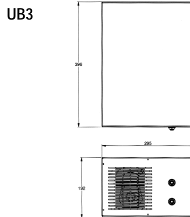
UNIT SUPPLIED WITH WATER CONNECTIONS
