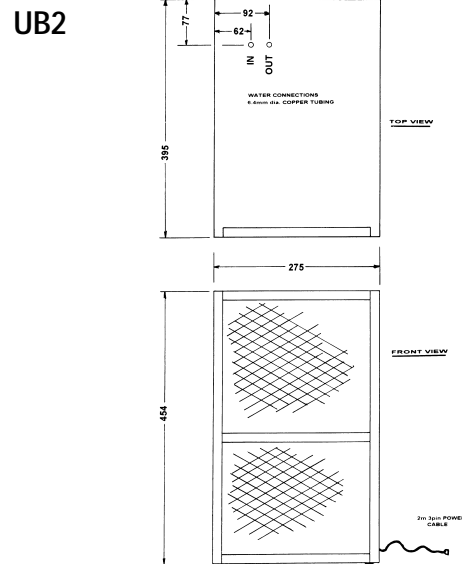
UNIT SUPPLIED WITH VENT & WATER CONNECTIONS
